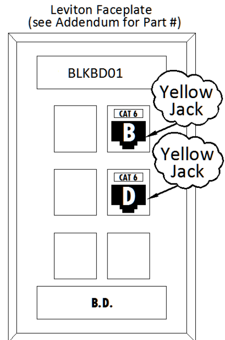
Blackboard Faceplate
