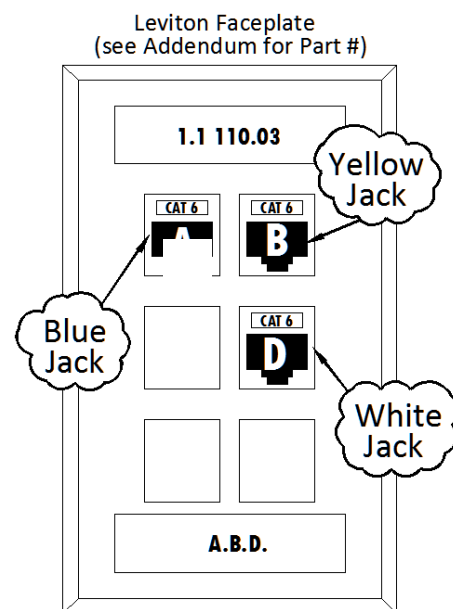
Standard/Intergrated Faceplate
